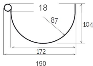
Section GRN133
